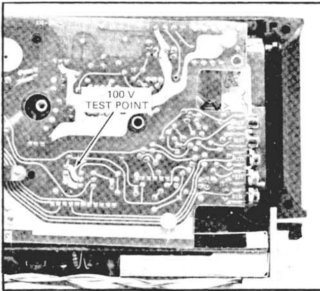
Fig. 4-2. Location of -100 V test point.
