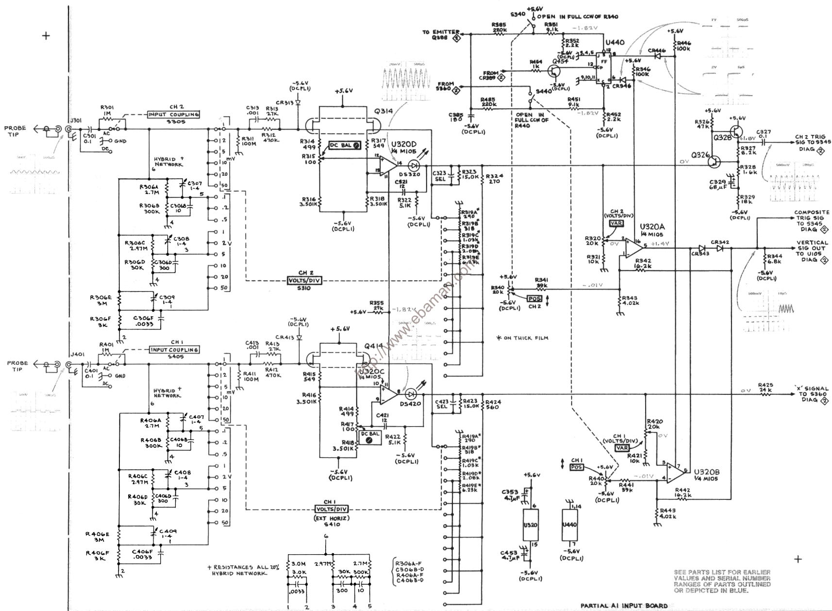
PARTIAL A1 INPUT BOARD
